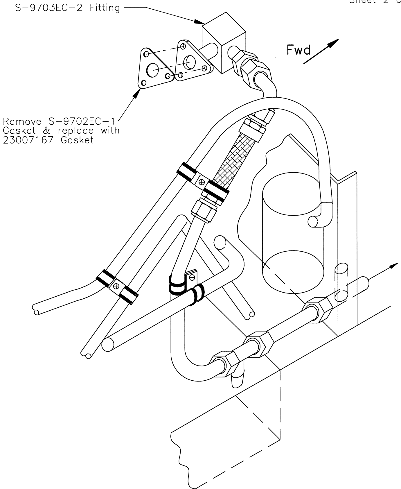
Figure 1: Engine Compartment Bleed Air System
